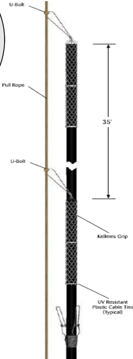
Illustration D: Pulling Detail
