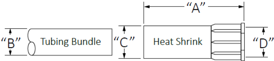
FAK-9: Sizing and Selection Chart
